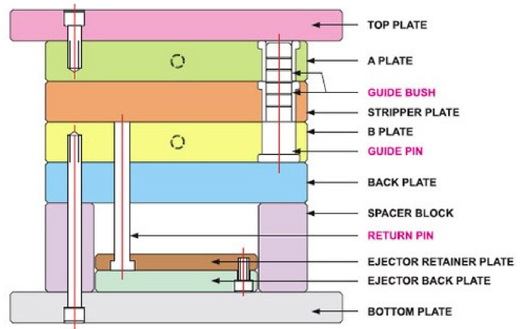
Mould Base
